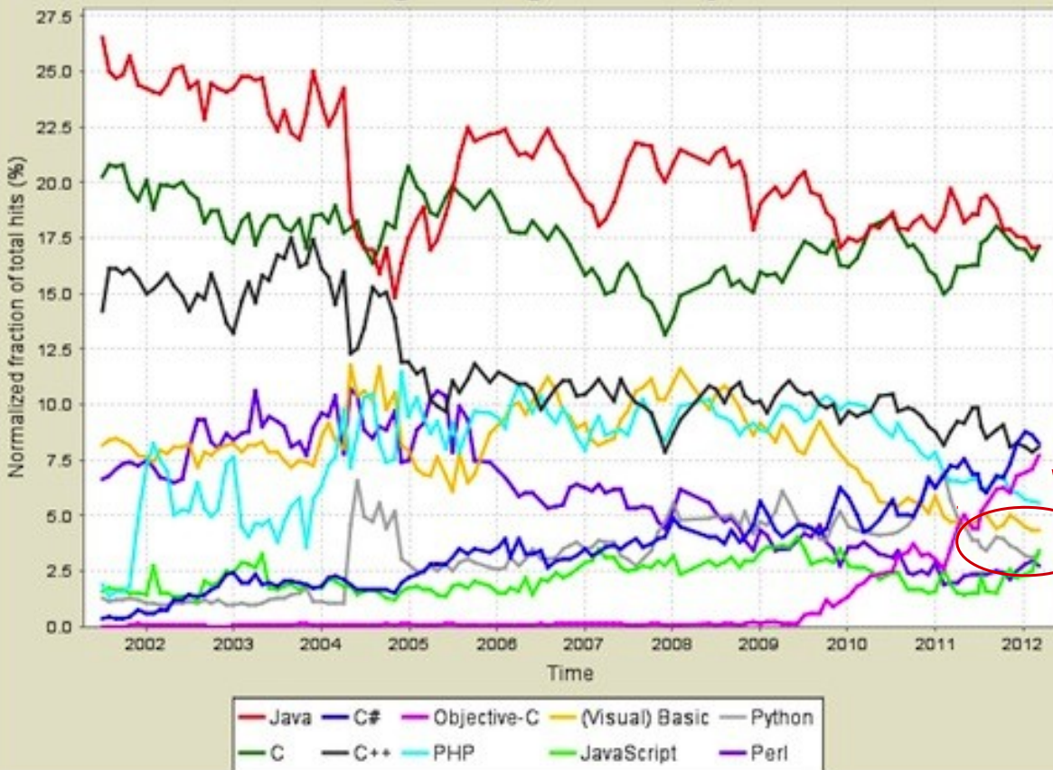
TIOBE Programming Community Index
